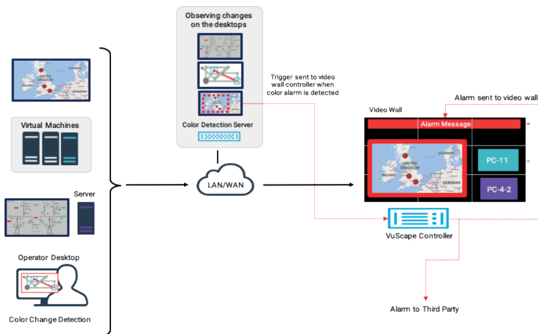
Diagram: Color Detection Workflow
